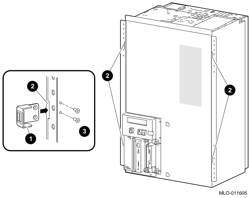
Figure 1: Installing the Latch Brackets
