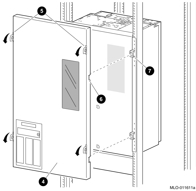
Figure 2: Installing the Front Bezel
