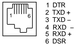
Figure A-2 Comm2—MMJ Port
